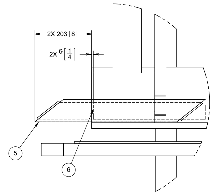
DETAIL F
