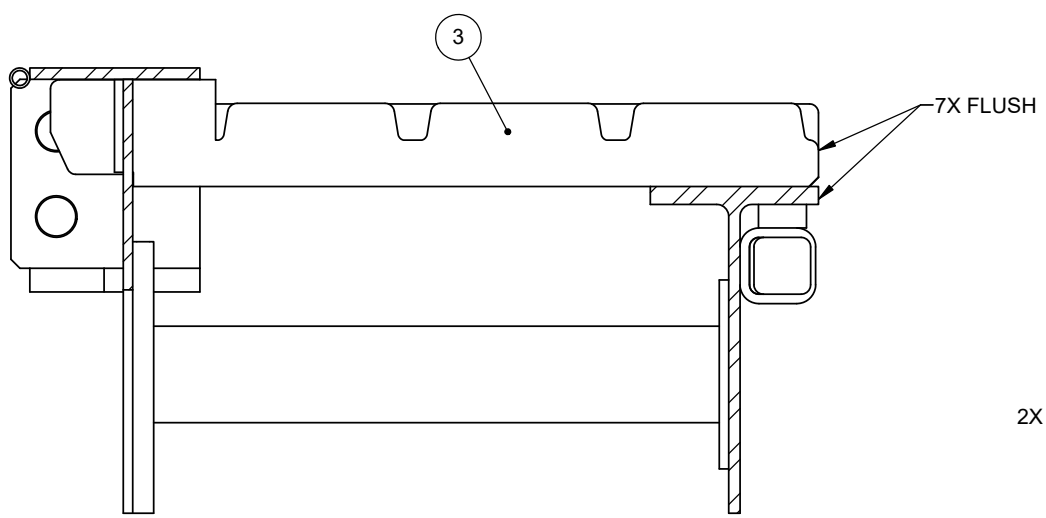
DETAIL D
