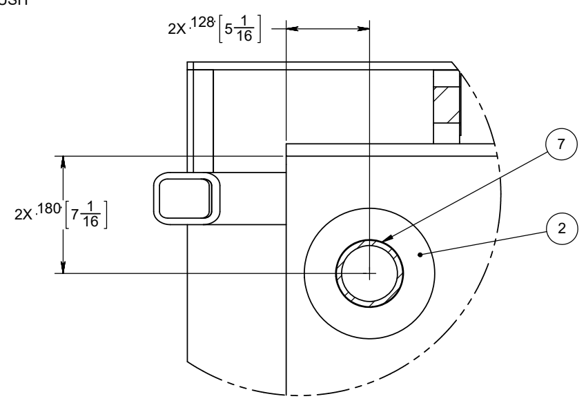
DETAIL E
